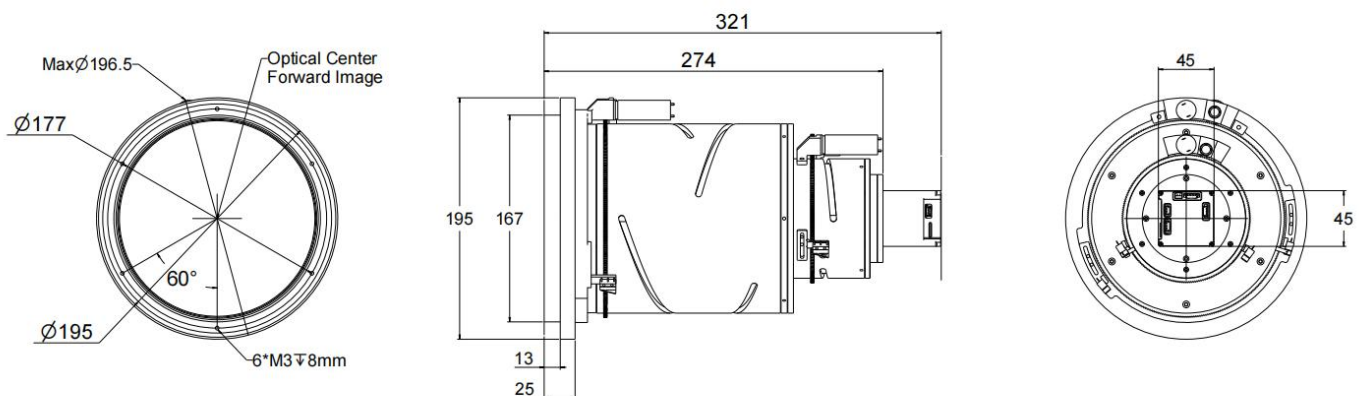
25~225mm Motorized Lens
