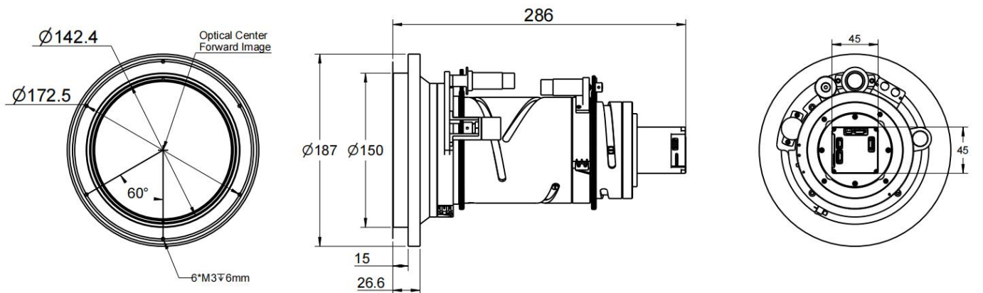
30~150mm Motorized Lens
